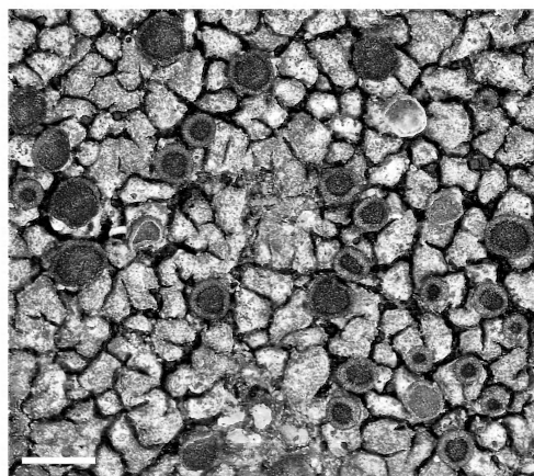
Fig. 1. Catillaria australitropicalis (holotype): habit. Scale bar: 0.5 mm.
